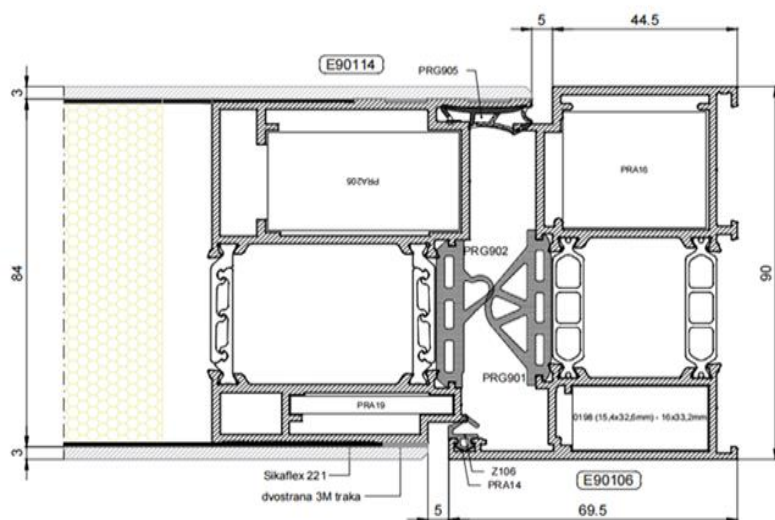
Obostrano skriveno krilo - Vanjsko otvaranje / Both-sided hidden sash - Outward opening
